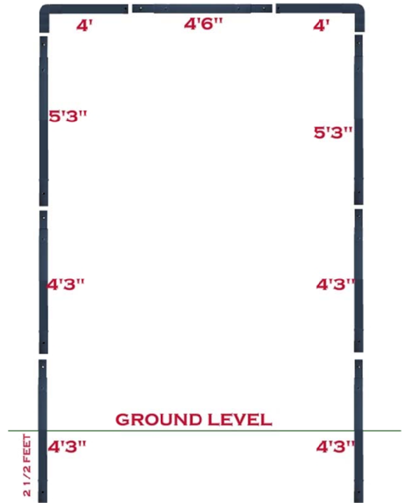
81157 12'6" X 14'3" FRAME SECTION FOR (12' X 12' NETTING)
